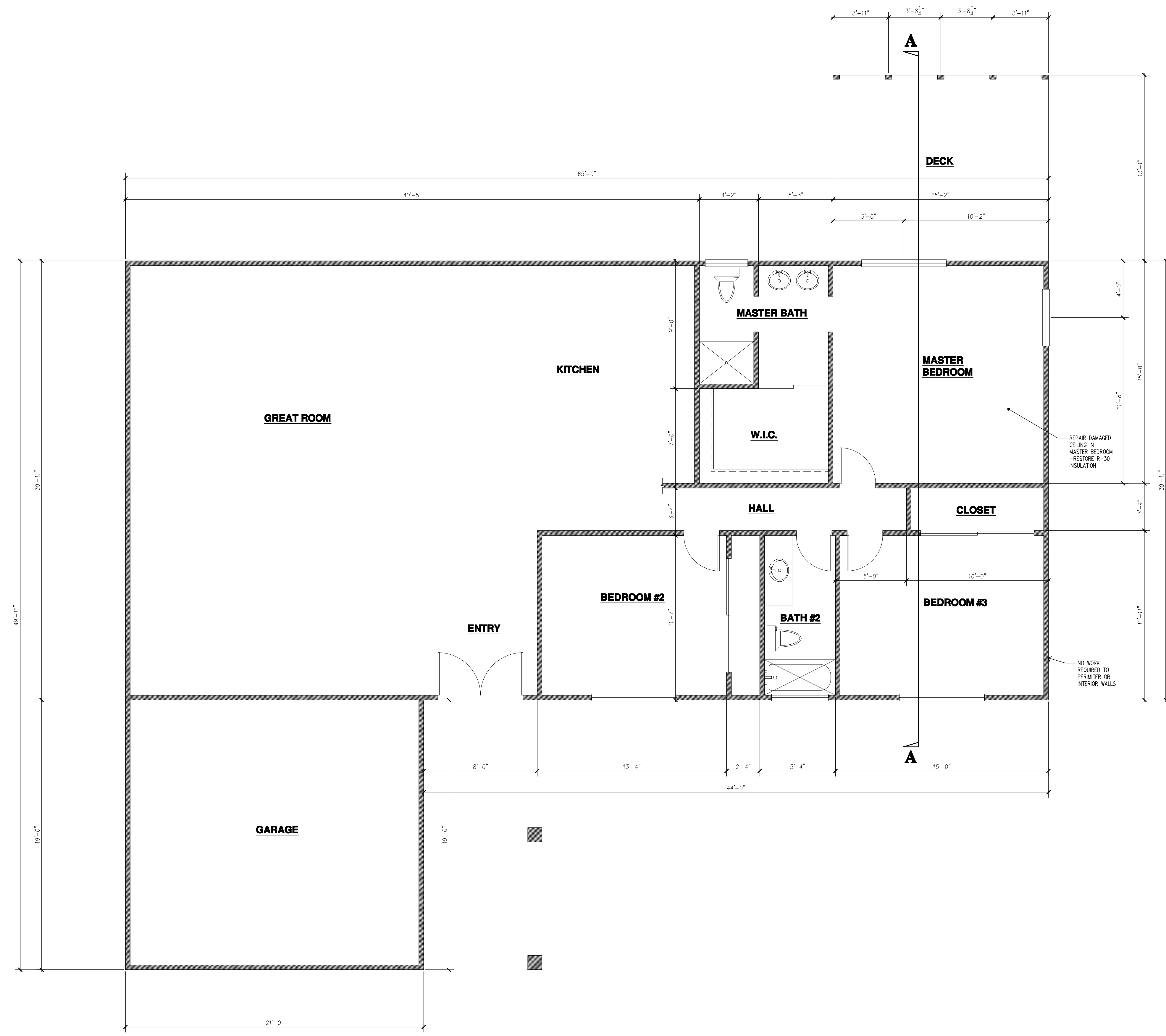
FLOOR PLAN
